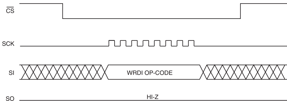
Figure 5. WRDI Timing
